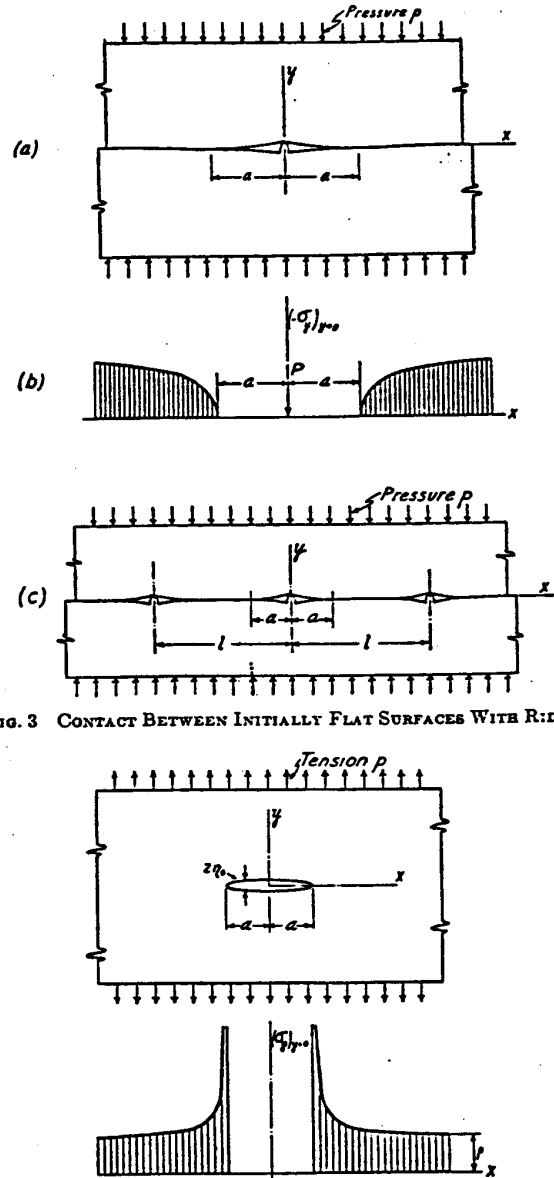
FIG. 4 INTERNAL CRACK
