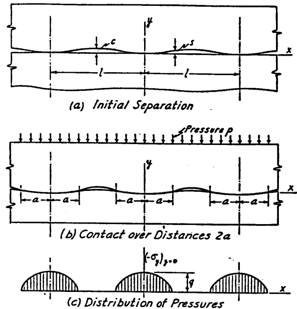
FIG. 1 BEARING PRESSURES THROUGH SLIGHTLY WAVED SURFACE
