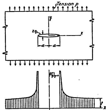
FIG. 4 INTERNAL CRACK
