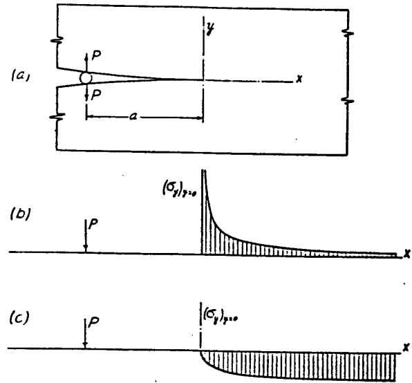
FIG. 5 CRACK OPENED BY WEDGE
